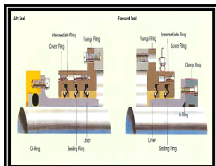
Stern Tube
