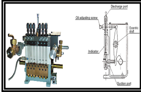
Cylinder Lubricator
