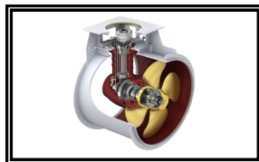
Bow Thruster
